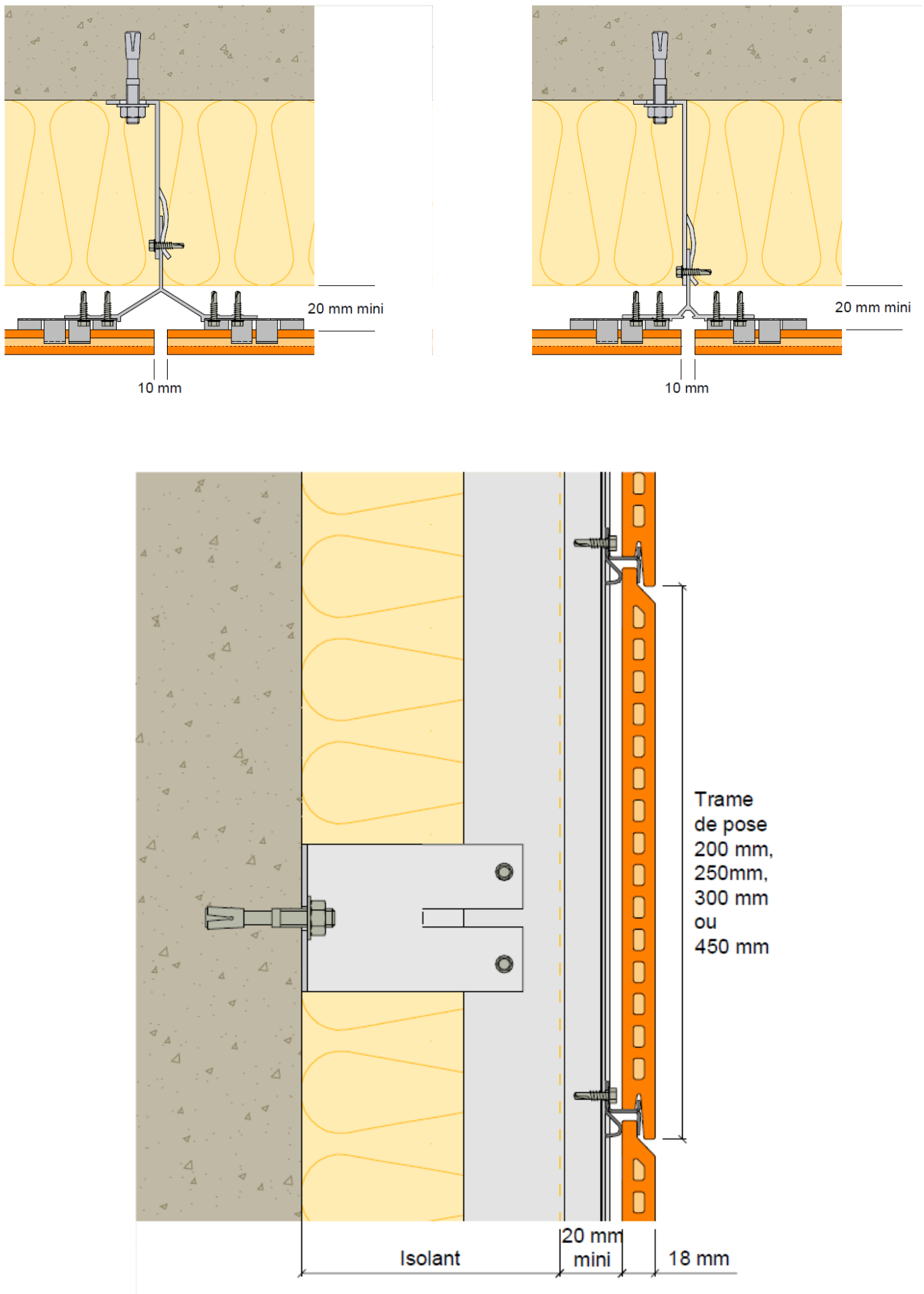
Figure 4: typical installation details (Y-section)
