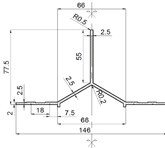
Y-profile section
