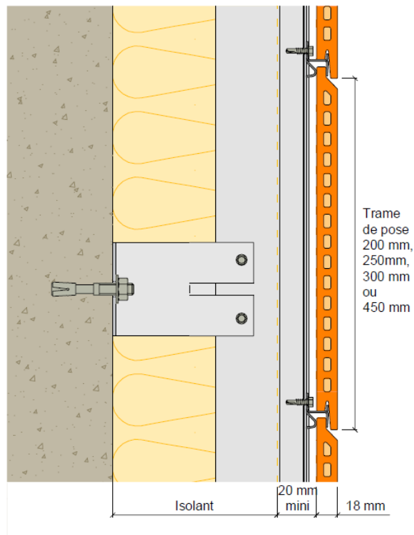
Figure 3: typical installation details (U-section)
